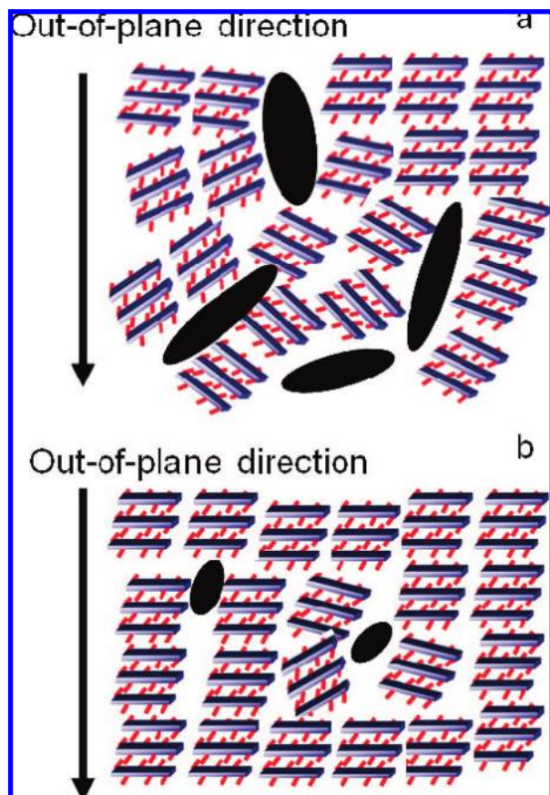
Figure 6. Schematic illustrations of (a) a high-RR P3HT–PCBM blend film containing many large PCBM crystallites, which cause the P3HT stacks to orient away from the out-of-plane direction, and (b) a low-RR P3HT–PCBM blend film with fewer and smaller PCBM crystallites and more ordered P3HT stacks.
